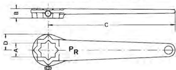
Standard wrench type 8K (Short)
